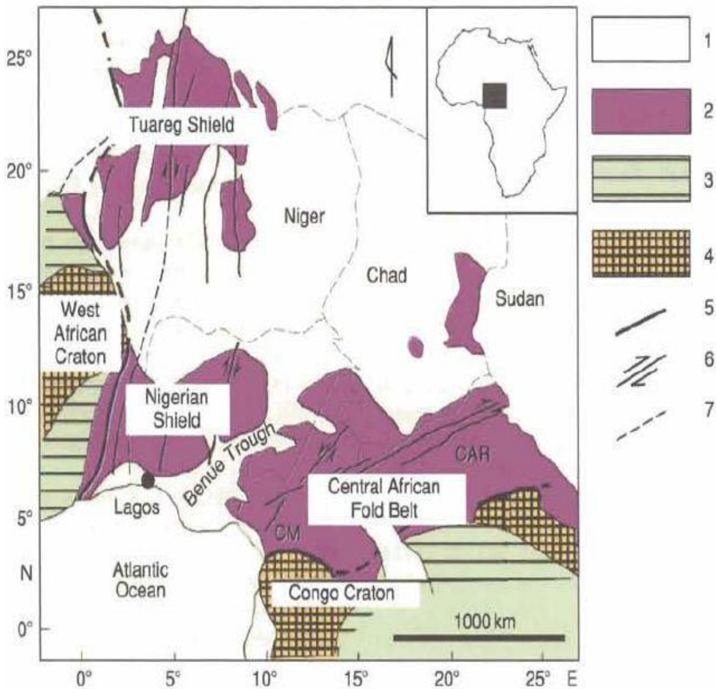
Fig. 5 : A Sketch Map Showing Pan-African Domains in West Central Africa. 1, Post-Pan-African Cover; 2, Pan-African Domains; 3, Pre-Mesozoic Platform Deposits; 4, Archaean to Palaeoproterozoic Cratons; 5, Craton limits; 6, Major Strike-slip Faults; 7, State Boundaries. CAR, Central African Republic; CM, Cameroun. (After Kroner and Stern, 2005).
