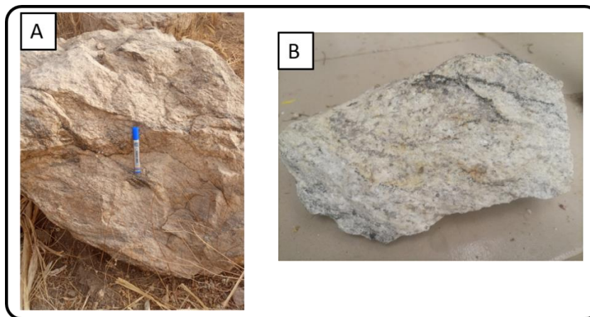
Plate.9: Photograph of showing (a) Field View of Schlieren type diatexite (B) Hand spacemen sample view
