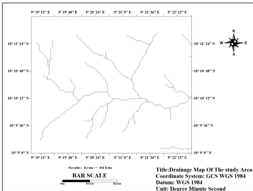
Fig. 3: Drainage map of the study area
