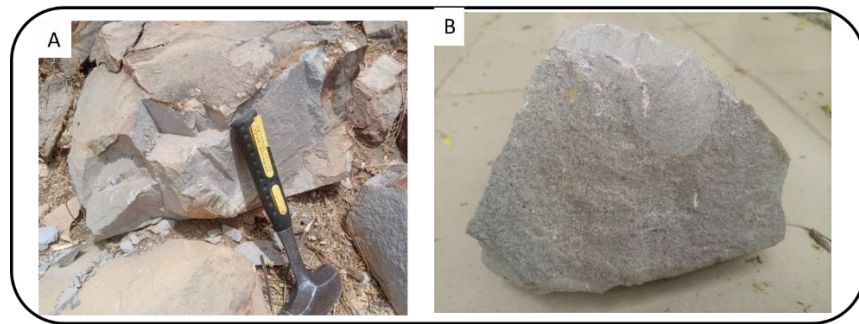
Plate.13: Photograph of showing (a) Field View of Rhyolite (B) Hand spacemen sample view of Rhyolite
