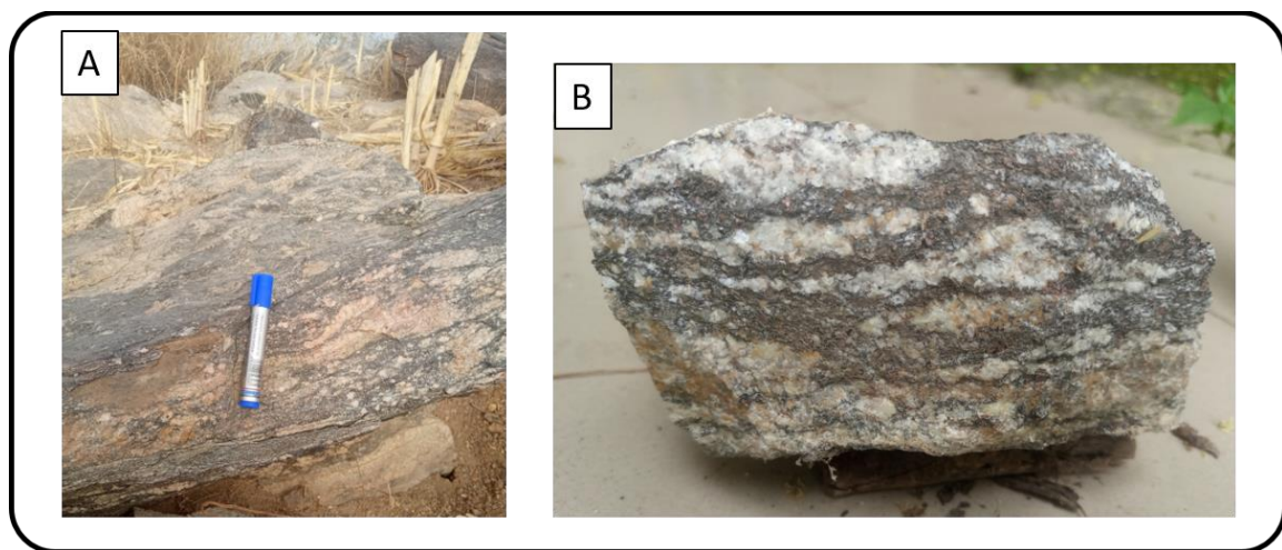
Plate.1: Photograph of showing (a) Field View of Banded Orthogneiss (B) Hand specimen
