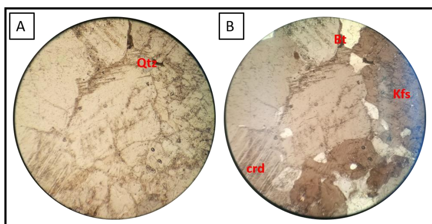
Plate.10: Photomicrograph of a sample of Schlieren type diatexite (a) under plane polarized light (b) under crossed polarized light. Qtz= quartz, Kfs=K-feldspar, Crd= Cordierite, Bt= Biotie.
