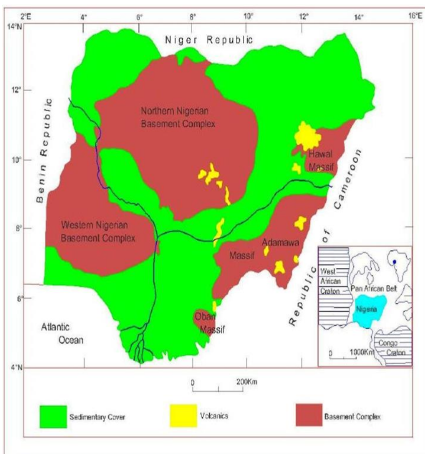
Fig.6: The Nigerian Basement Complex Provinces. (After Haruna, 2016)
