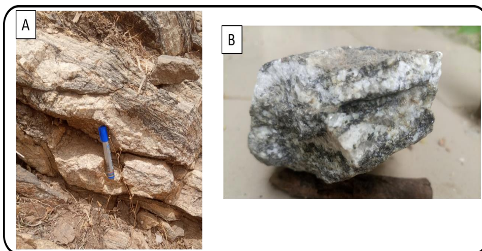
Plate.3: Photograph of showing (a) Field View of Banded Orthogneiss (B) Hand spacemen
