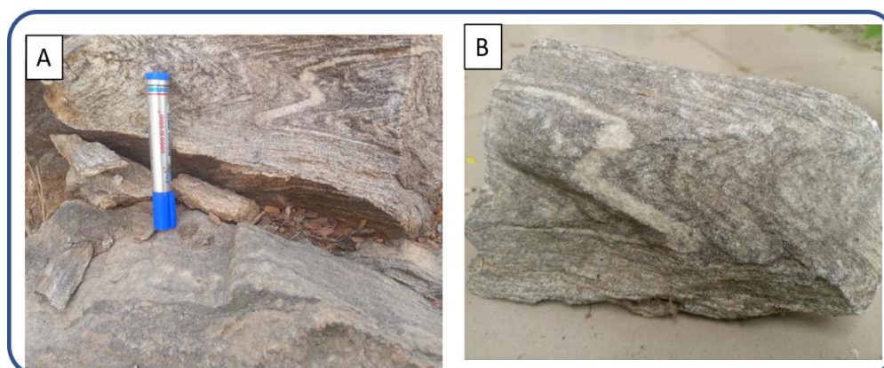
Plate.5: Photograph of showing (a) Field View of Stromatic Metatexite (B) Hand spacemen sample
