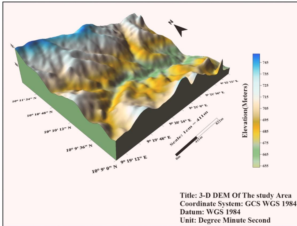
Fig. 2: 3-D Digital Elevation map of the study area
