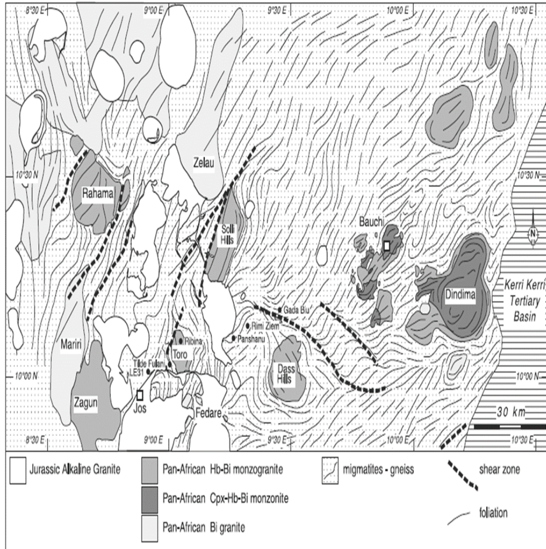
Fig. 7: Geological Map of the Jos–Bauchi Area. Foliations Compiled from Field Data, SLAR Images and Previous Maps. Source: Wright, (1971).
