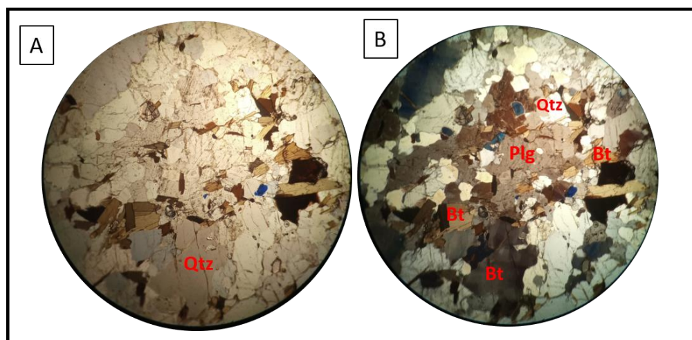
Plate.2: Photomicrograph of a sample of banded orthogneiss (a) under plane polarized light (b) under crossed polarized light. Qtz= quartz, Bt= Biotite, Plg= Plagioclase.
