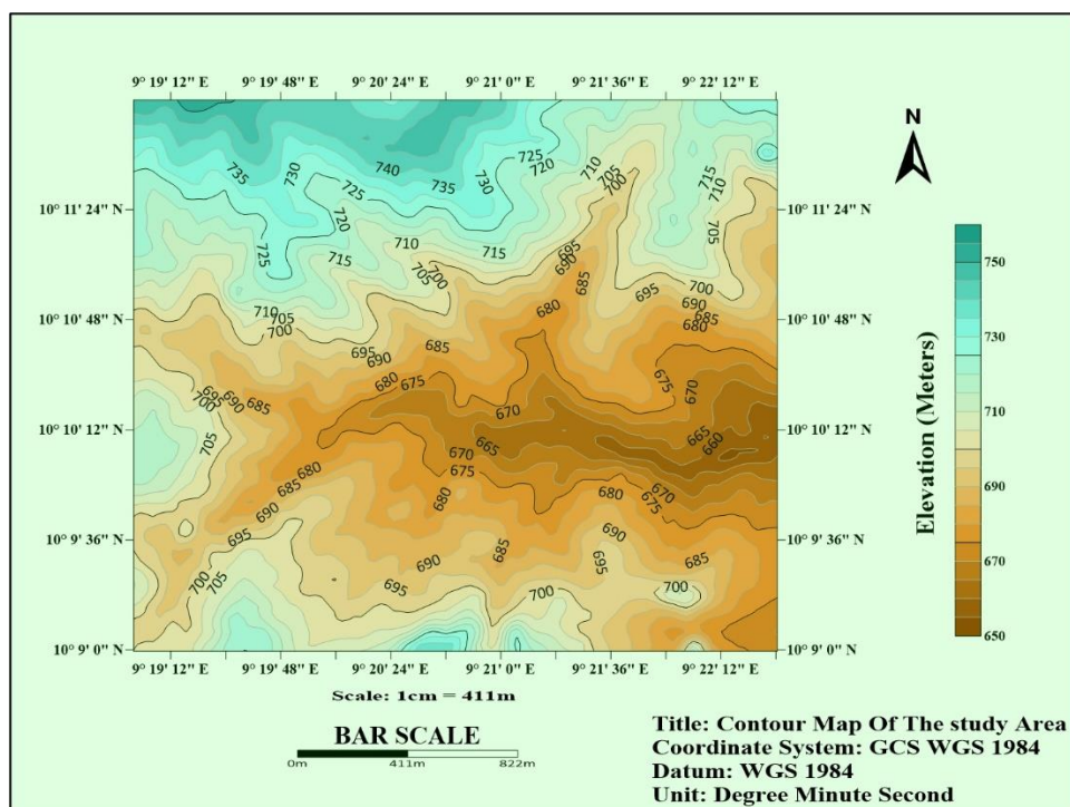
Fig. 4: Contour map of the study area
