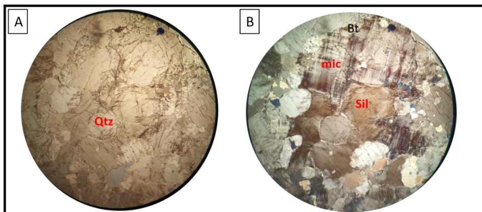
Plate.8: Photomicrograph of a sample of Schlieren type diatexite (a) under plane polarized light (b) under crossed polarized light. Qtz= quartz, Mic= Microcline, Sil= Sillimanite.
