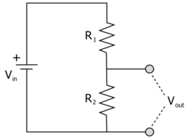
Figure 1.2: Voltage divider
