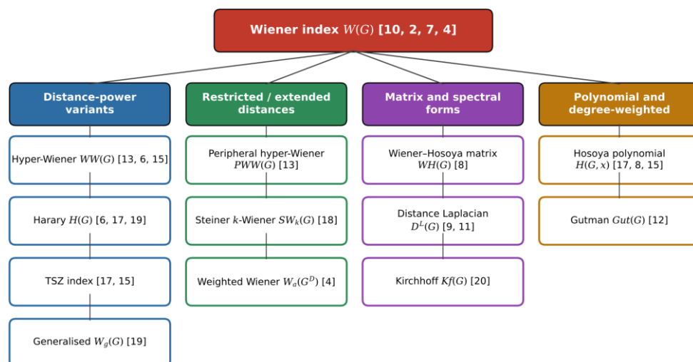
Figure 2. Taxonomy of the Wiener-index variants listed in Table 1, grouped into four families; the bracketed numbers are the references given for each variant in Table 1.
