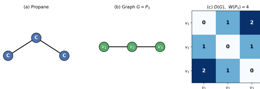
Figure 1. The relationship among propane, its hydrogen-suppressed graph G = P_3 , and the corresponding 3 \times 3 distance matrix D(G) . The Wiener index W(P_3) = 4 is the sum of the upper-triangular entries of D(G) .
