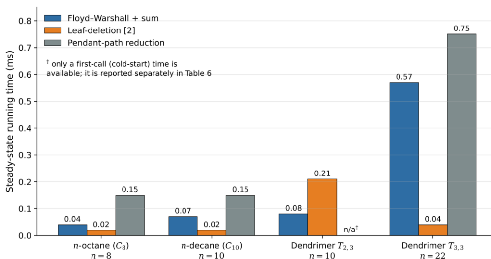
Figure 5. Steady-state Wiener-index computation times (ms) for the graphs in Table 6; first-call (JIT-affected) times are excluded.
