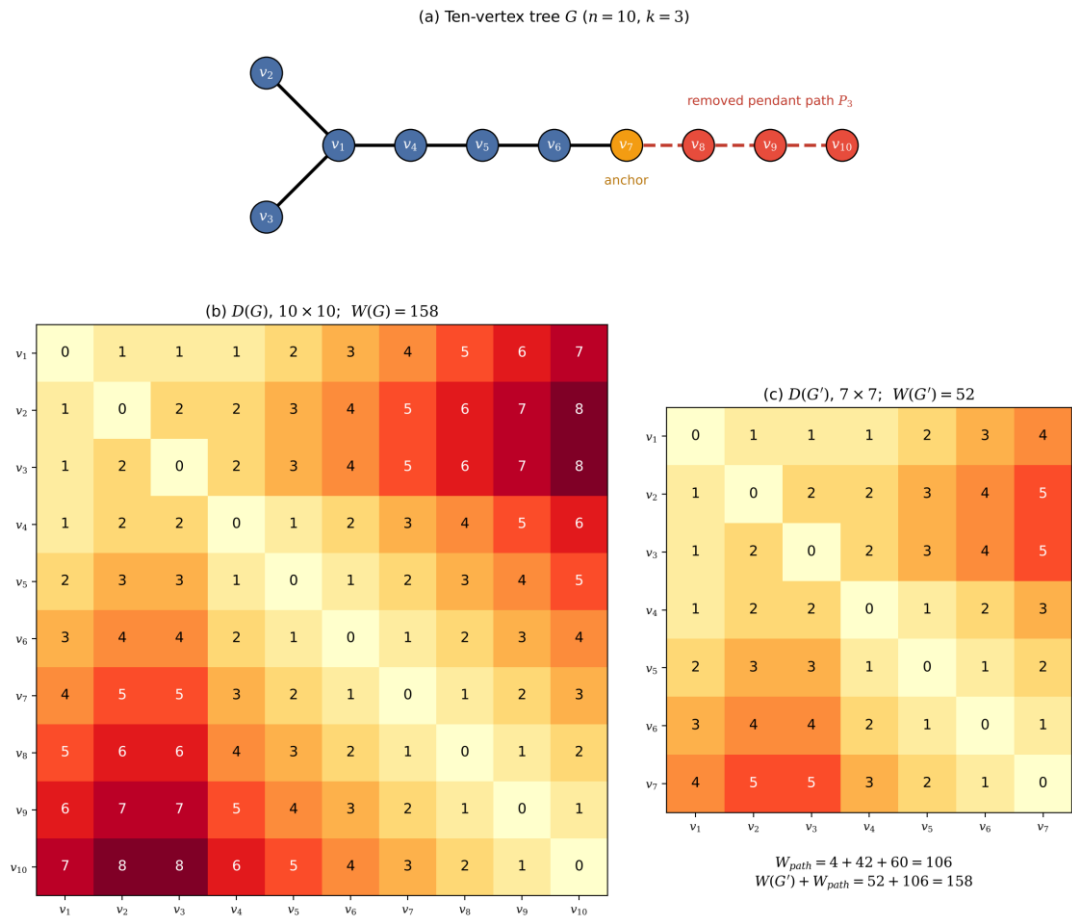
Figure 3. The ten-vertex reference tree under the proposed cut: (a) the tree G (edge list in Section 6.3), with anchor v_7 and removed pendant path v_8v_9v_{10} ; (b) the 10 \times 10 distance matrix D(G) ; (c) the 7 \times 7 distance matrix D(G') of the reduced tree.
