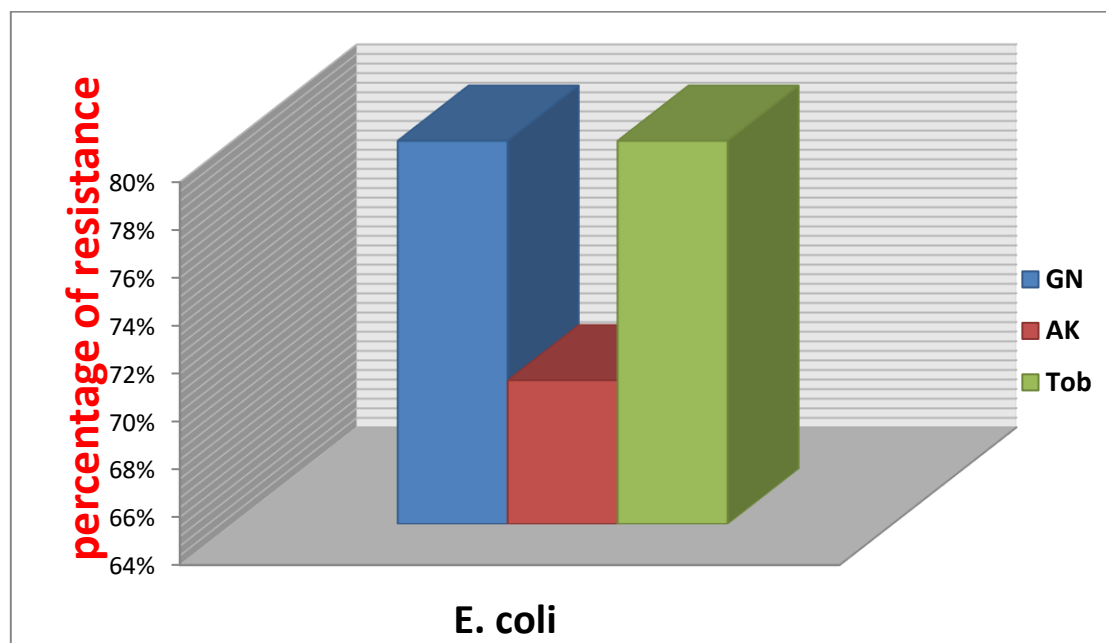
Figure 1: the percentage of E. coli resistance to AG
