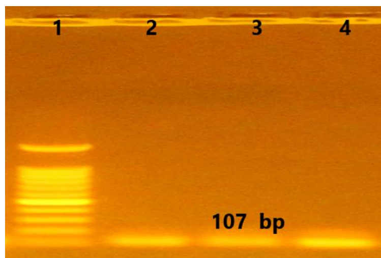
Figure 3: gel electrophoresis for acrB PCR products (107 bp) as shown that line 1 refer to DNA ladder and three other line (2, 3 and 4) as positive results.
