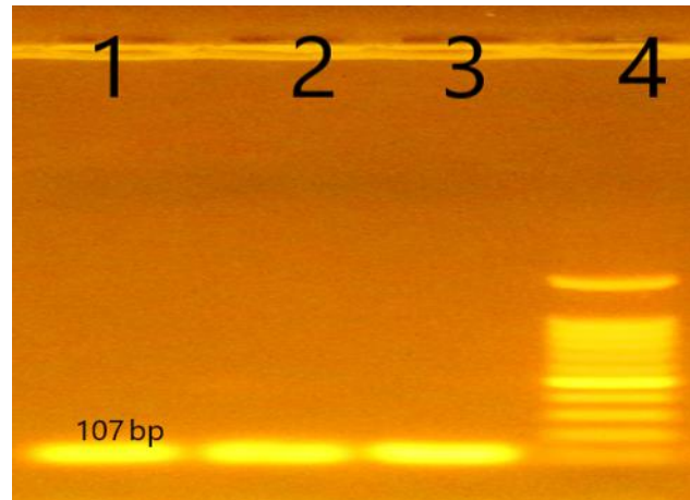
Figure 2: agarose gel electrophoresis for acrA PCR products (107 bp). Line 4 as DNA ladder (1000 bp), three line 1, 2 and 3 as a positive result.
