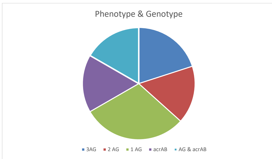
Figure 4: phenotype and genotype detections
