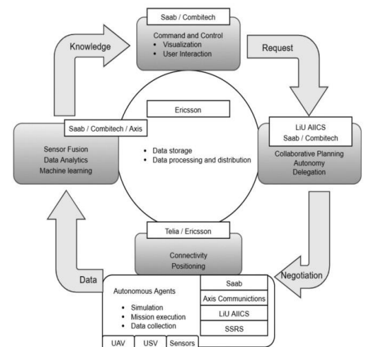
Fig. 2. Overview of the system (adapted from WARA-PS internal presentation material).
